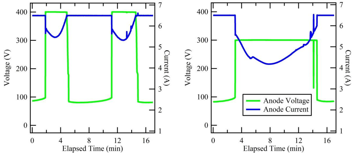
Figure 9. The heating portion of two different discharge cycles with a current limit of 6.5 amps. Left: Discharge cycle with a 400 volt voltage limit. Right: Discharge cycle with 300 volt voltage limit.
