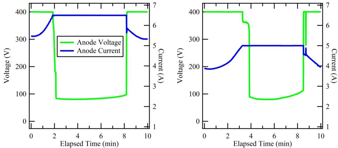
Figure 8. Cooling portions of two discharge cycles with different current limits. Left: discharge cycle current-limited to 6.5 amps with a minimum power of 523 W. Right: discharge cycle current limited to 5 amps with a minimum power of 400 W.
